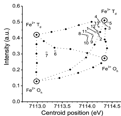
Figure 3. Plot of the pre-edge integrated intensity (area) and the centroid position (area-based average position) extracted from HERFD-XANES spectra of reference compounds representative of Fe 2+ and Fe 3+ in O_h and T_d states (large circles), their binary linear combinations (filled diamonds) and the Fe-ZSM-5 catalyst under reaction conditions numbered according to Table 1 (open squares) used to estimate Fe oxidation state and coordination geometry.
