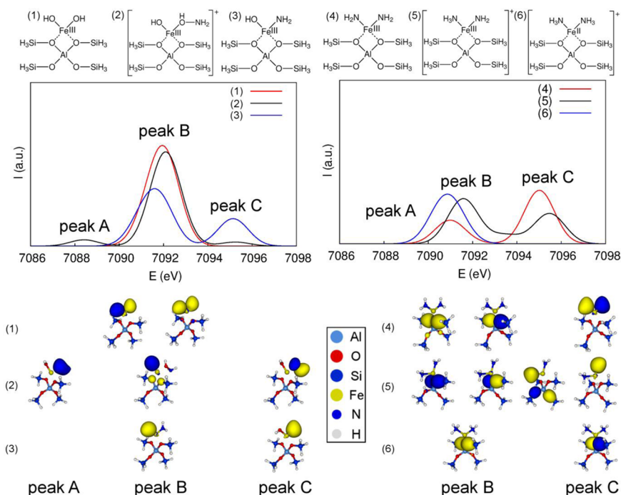
Figure 6. Top: Lewis structures of molecular models (1)–(6) considered in DFT calculations. Middle: calculated V2C XES K\beta'' spectra for these models. Bottom: The orbitals from which the main contribution to peaks A–C originates, shown as isosurface plots.
