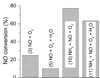
Figure 1. Conversions of NO measured during XAS/XES data acquisition for NO oxidation and SCR of NO with and without water. Conditions: 1000 ppm of NO, (1000 ppm of NH 3 ), 5% O 2 (approximately 1.5% H 2 O) and pure He as balance.
